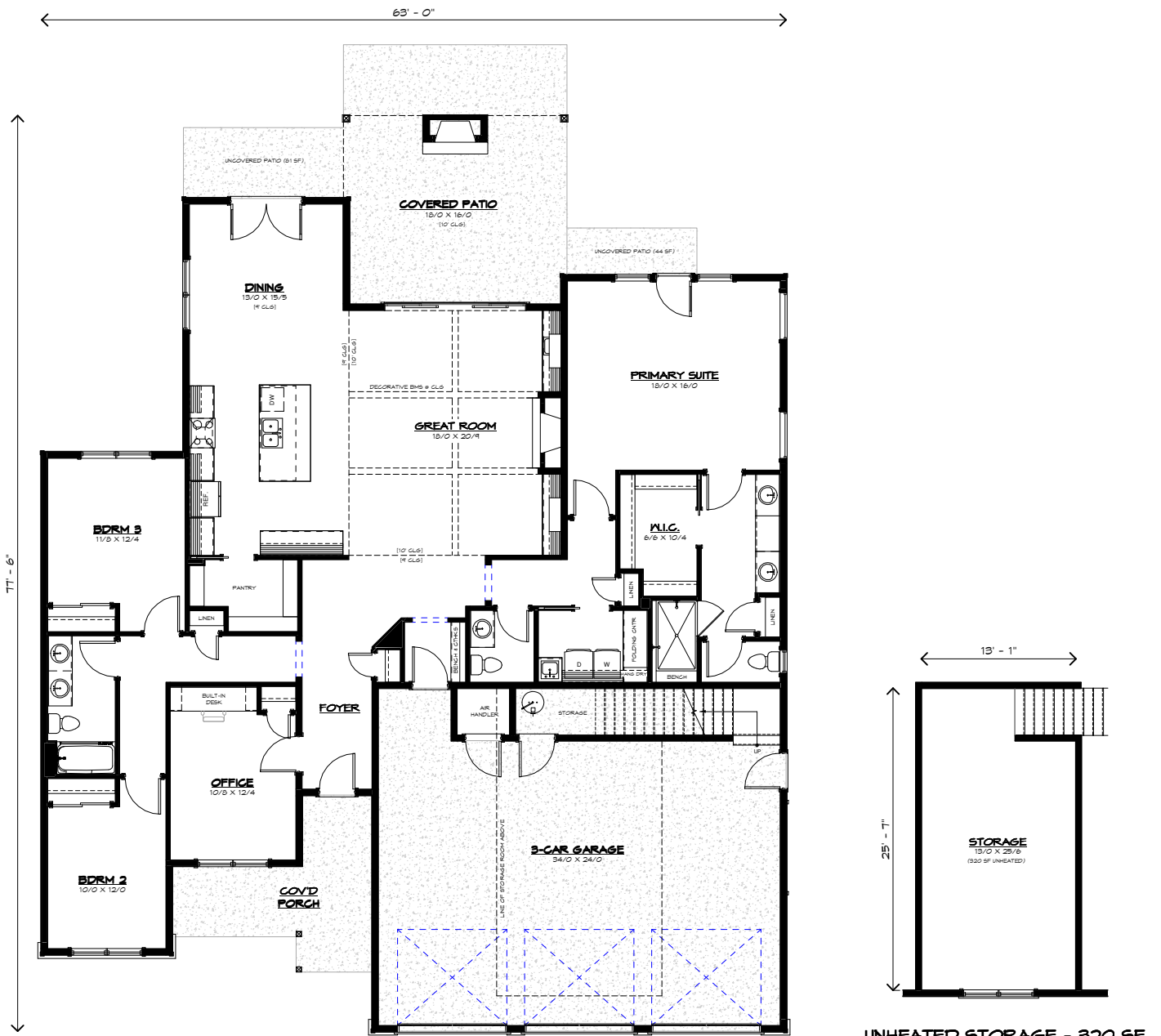
MAIN FLOOR - 2540 SF
