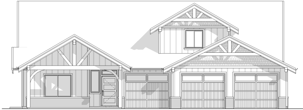
MCKENZIE PLAN - 2557 SQFT
