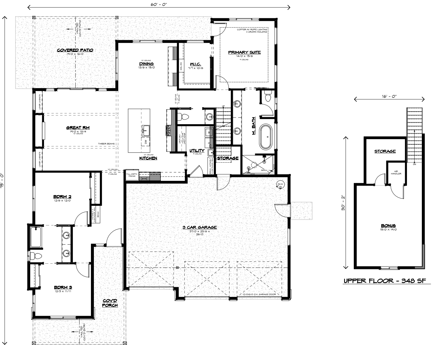
MAIN FLOOR - 2209 SF
