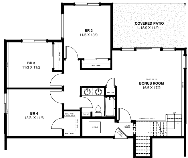
LOWER FLOOR PLAN 1/4" = 1'-0"
