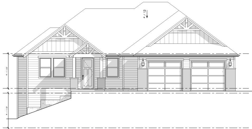
Front Elevation - 2986 SF 1/4" = 1'-0"
