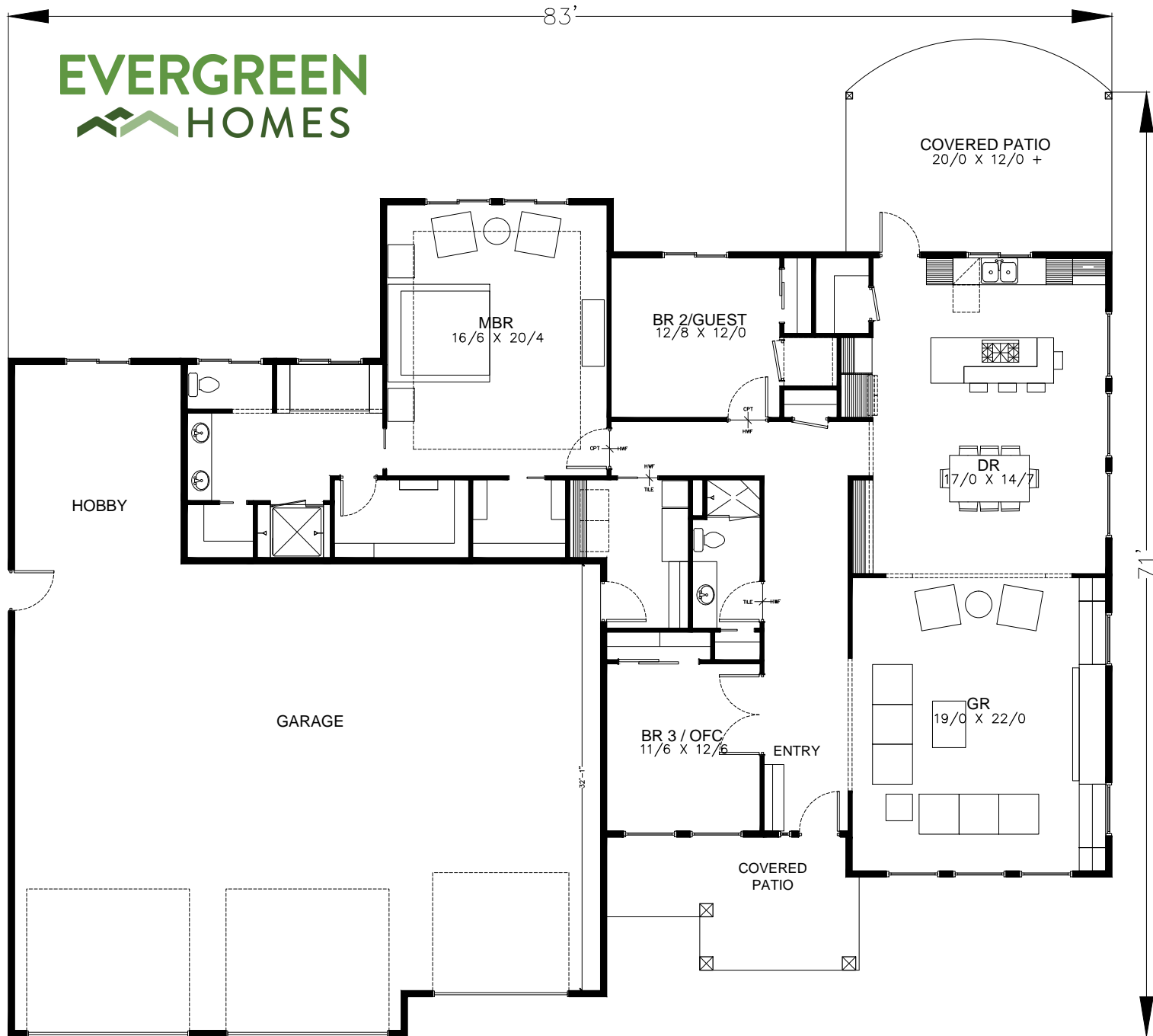
PLAN 2442 83' W X 71' D MAIN LEVEL, 2442 SF, 9'10"6" Ceiling Evergreen Homes NW Copyright 2017
