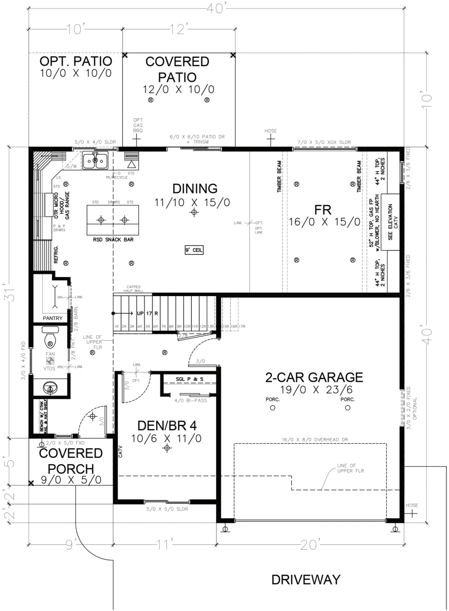
SP 8 SPEC PLAN 2084 40' W x 50' D MAIN LEVEL, 1027 SF, 9' Ceiling Evergreen Homes NW Copyright 2015
