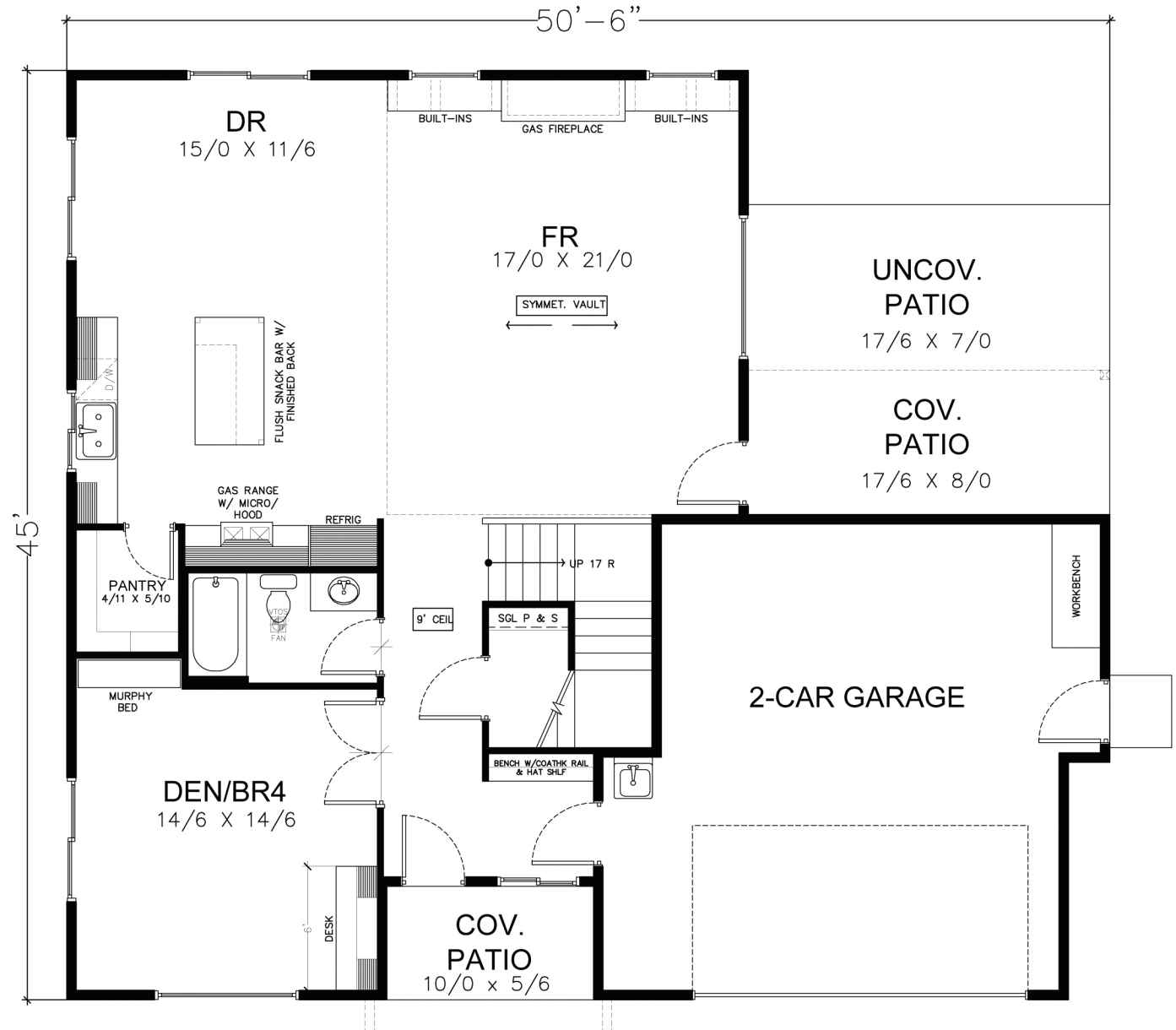
PLAN 2509 50'6" W x 45' D MAIN LEVEL, 1297 SF, 9' Ceiling Evergreen Homes NW Copyright 2014
