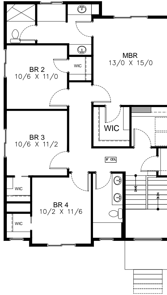
PLAN 2333 29' W X 46'6" D
