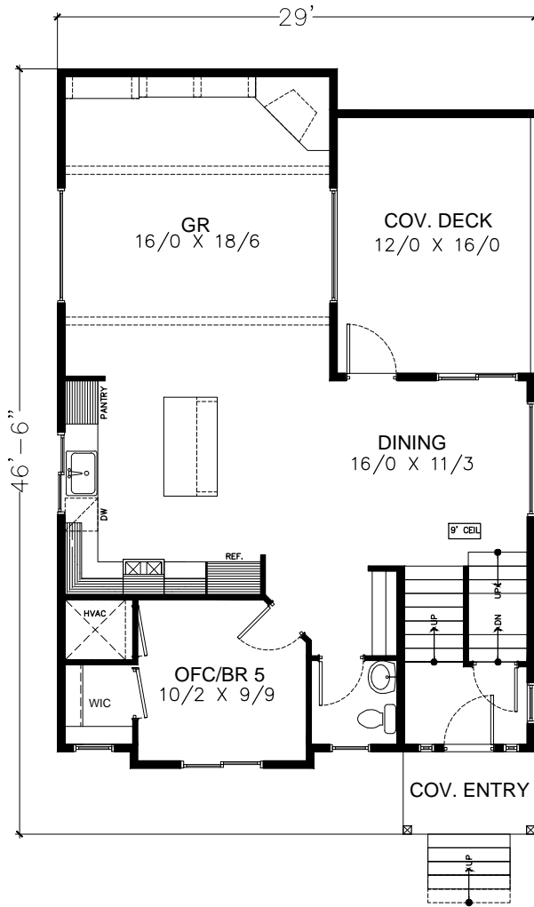
PLAN 2333 29' W X 46'6" D
