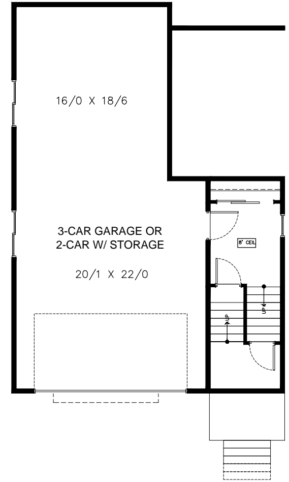
PLAN 2333 29' W X 46'6" D
